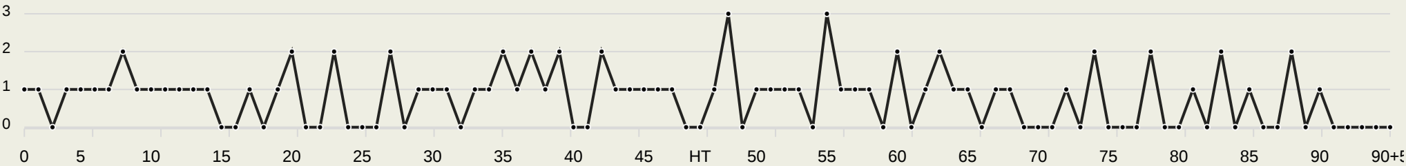
Auckland City FC GK Involvement Timeline
